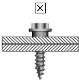
Under driven. Requires tightening
