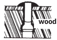
GROOVED RIVET Grooves improve holding strength
